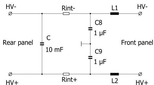
Abb. 8. Common Mode: CM / 2 x 1μF. Jumper (orange) auf „JP2-“ und „JP2+“ stecken. Fig. 8. Common Mode: CM / 2 x 1μF. Plug jumpers (orange) on "JP2-" and "JP2+".
