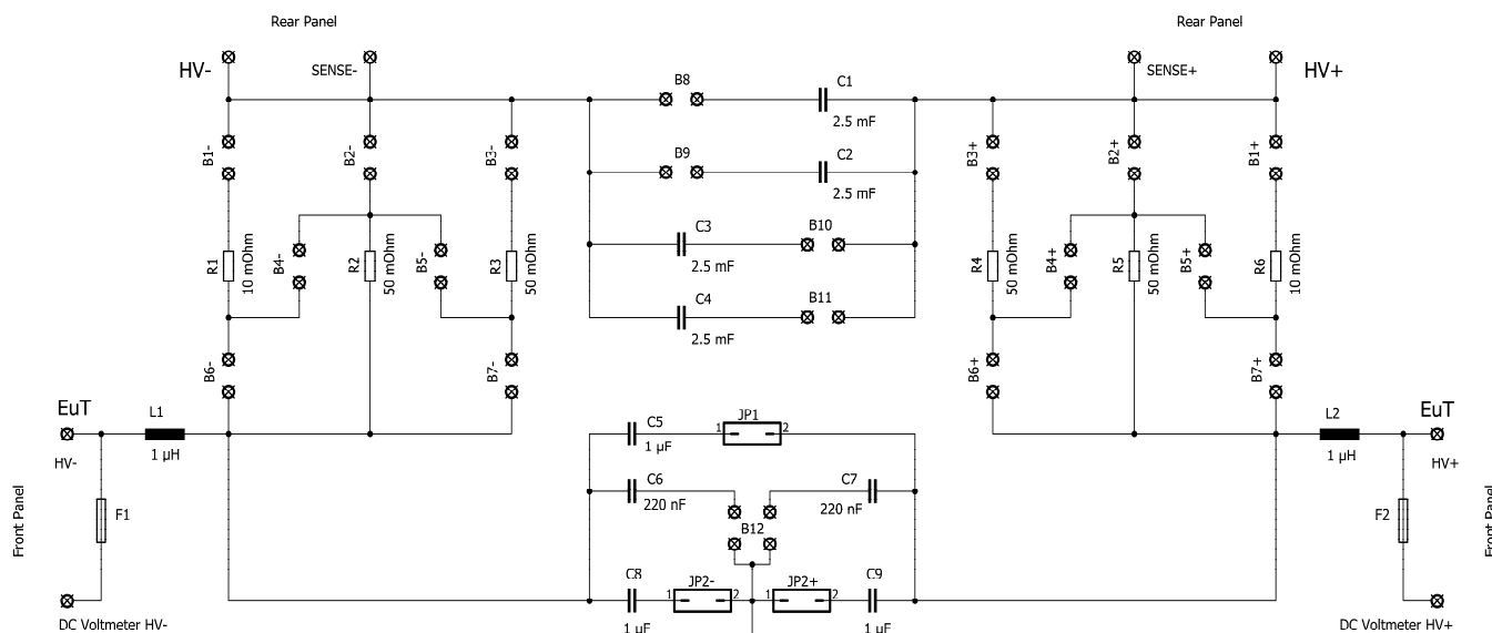
Abb. 2. Schaltplan BNB 8656. Fig. 2. Circuit of BNB 8656.
