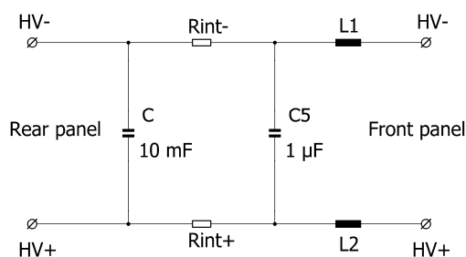
Abb. 7. Differential Mode: DM / 1μF. Jumper auf „JP1“ stecken. Fig. 7. Differential Mode: DM / 1μF. Plug jumper on "JP1".
