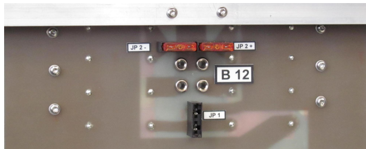
Abb. 8. Common Mode: CM / 2 x 1μF. Jumper (orange) auf „JP2-“ und „JP2+“ stecken. Fig. 8. Common Mode: CM / 2 x 1μF. Plug jumpers (orange) on "JP2-" and "JP2+".
