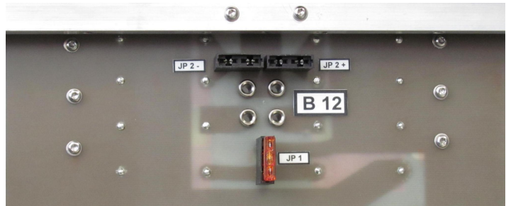
Abb. 7. Differential Mode: DM / 1μF. Jumper auf „JP1“ stecken. Fig. 7. Differential Mode: DM / 1μF. Plug jumper on "JP1".
