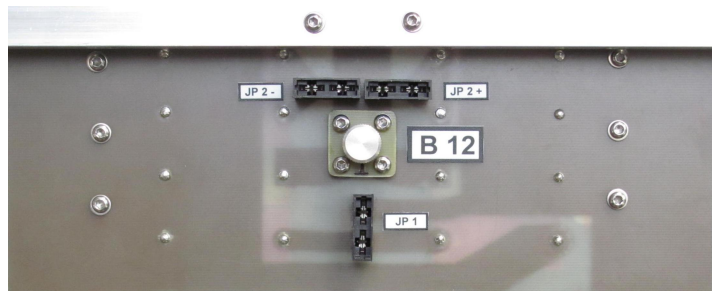
Abb. 10 Common Mode: CM / 2 \times 0.22\mu\text{F} . Brücke B12 einstecken (ISO 21498-2:2021-03). Fig. 10. Common Mode: CM / 2 \times 0.22\mu\text{F} . Plug in bridge B12 (ISO 21498-2:2021-03).
